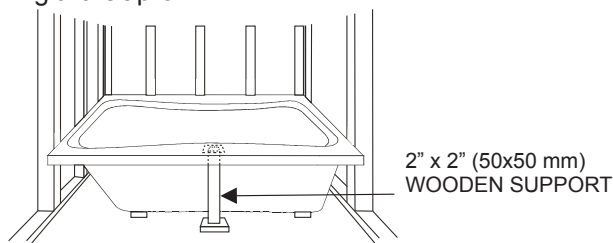
FIGURE 1 - ALCOVE INSTALLATION
